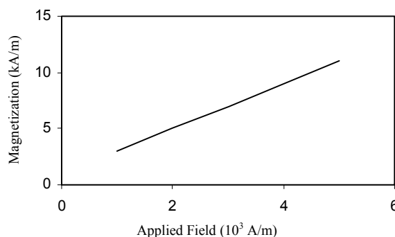
Fig. 1 Magnetization as a function of applied field.
